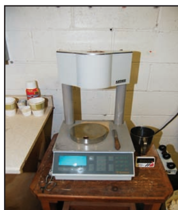
Kayness Melt Indexer
